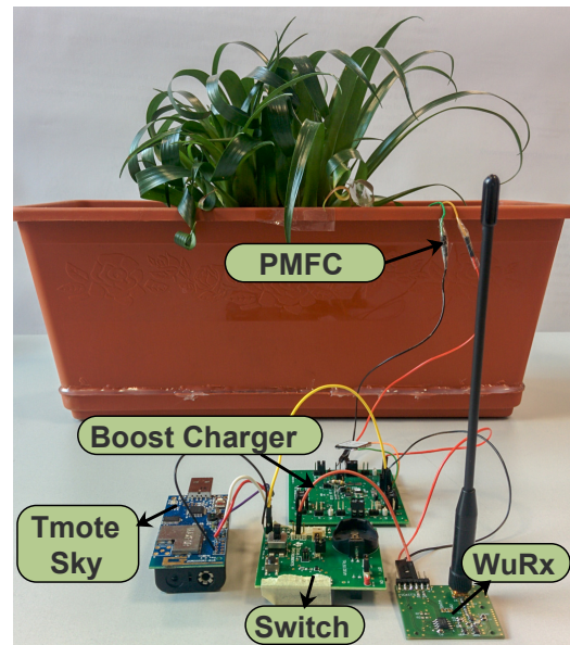
Figure 1: Laboratory setup of the plant microbial fuel cell powered sensing system showing different modules.
