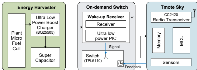
Figure 2: Overall architecture of the wake-up receiver triggered on-demand sensing unit. When a trigger is received, the switch closes to connect the sensing and transmitting node to the PMFC-based energy harvested power supply. Black lines indicate the power supply while blue indicates trigger signaling.
